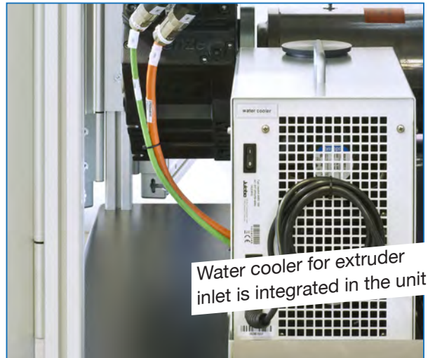
No clumping from adhesive granulates due to water cooling in extruder inlet
